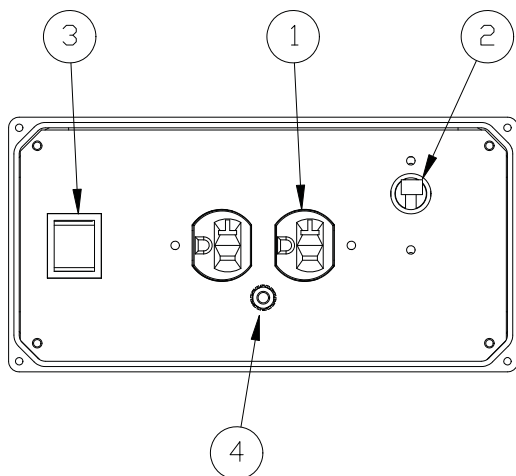
Figure 1 - Control Panel
